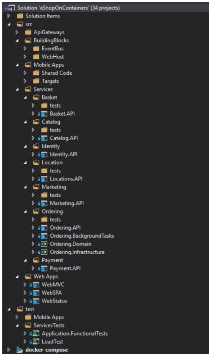
Figure 2-4. Projects in Visual Studio solution.
