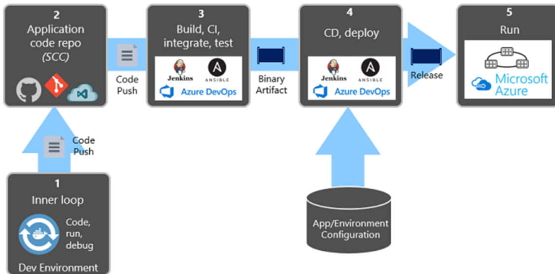
Figure 1-8. Deployment steps in a CI/CD Pipeline
