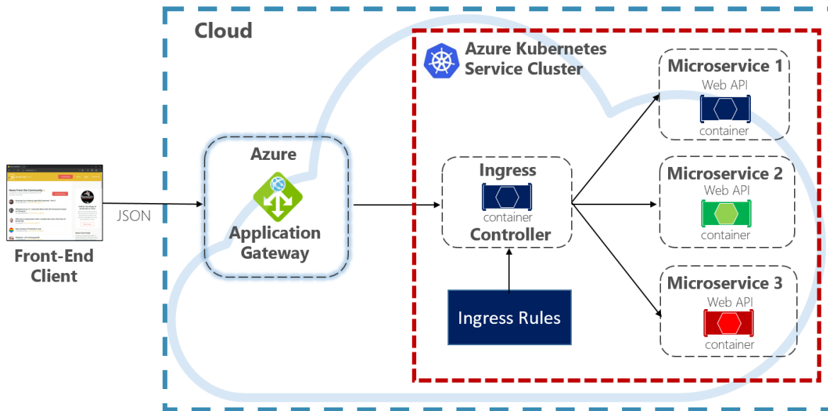
Figure 4-5. Application Gateway Ingress Controller
