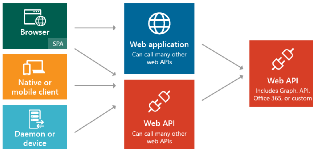
Figure 8-1. Application types and scenarios.
