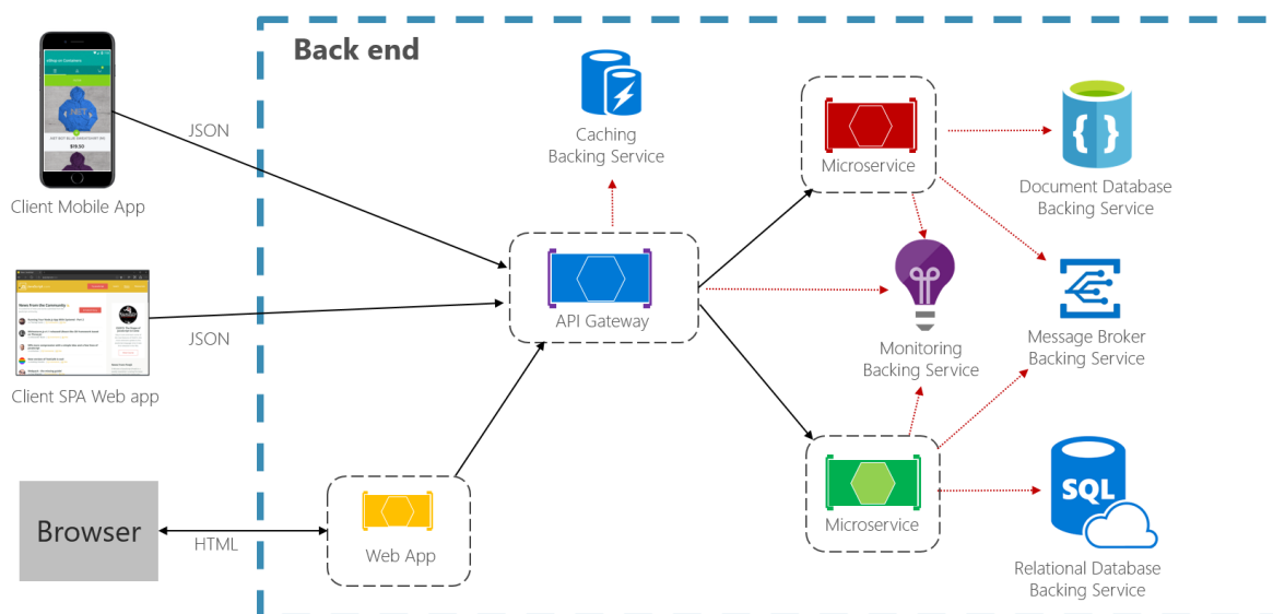
Figure 6-1. Distributed cloud-native environment
