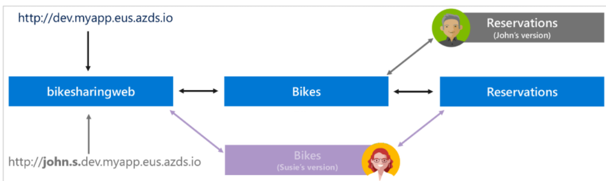
Figure 2-8. Developer John deploys his own version of the Reservations microservice and tests it without conflicting with other developers.
