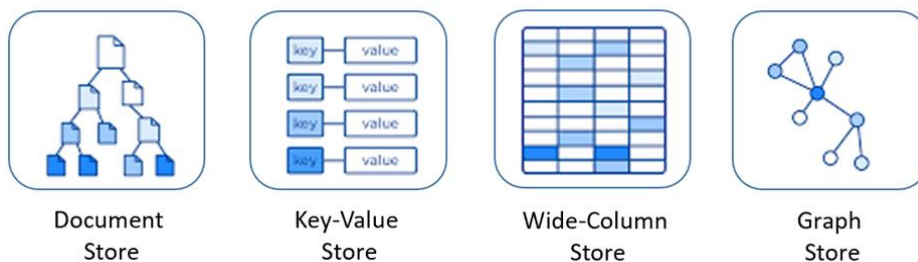
Figure 5-9: Data models for NoSQL databases
