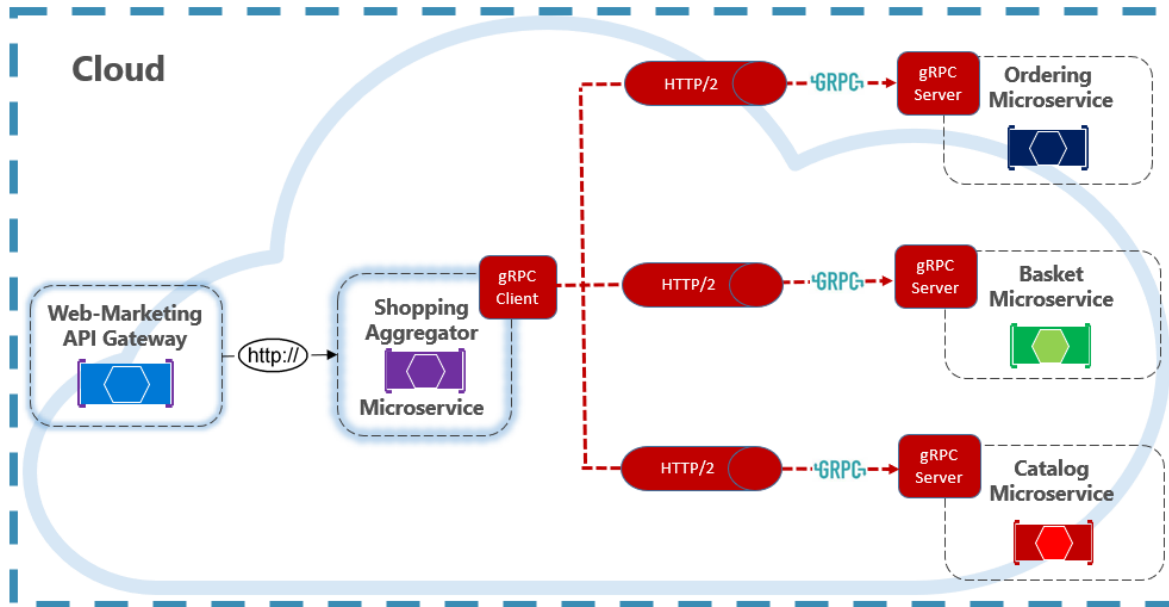
Figure 4-23. gRPC in eShop on Containers
