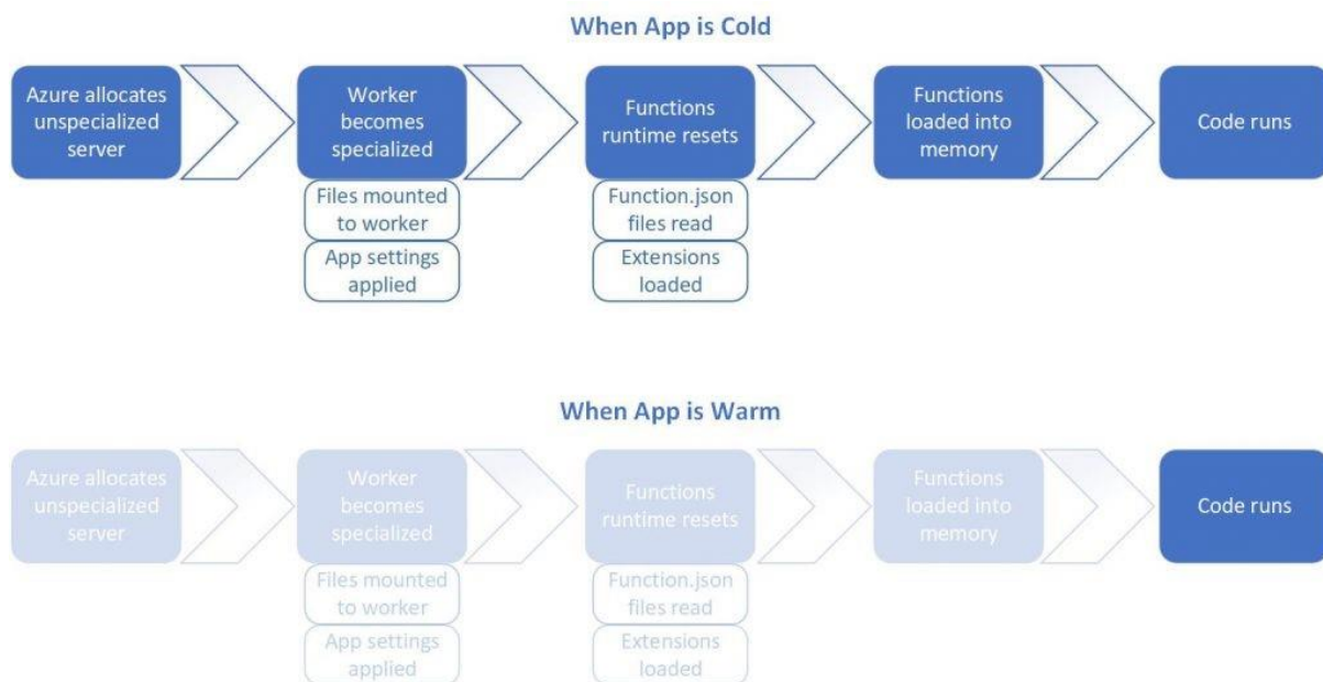
Figure 3-10. Cold start versus warm start.
