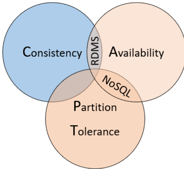
Figure 5-10. The CAP theorem
