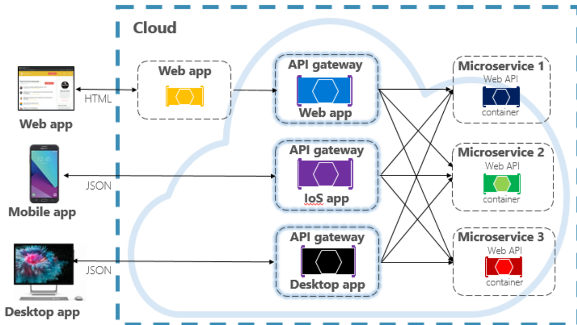
Figure 4-4. Backend for frontend pattern
