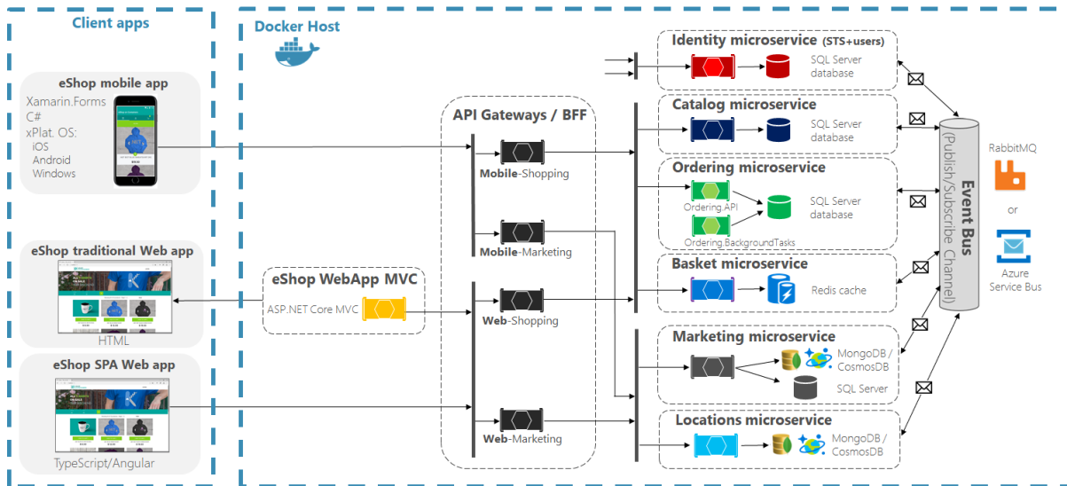
Figure 2-2. eShopOnContainers reference application development architecture.
