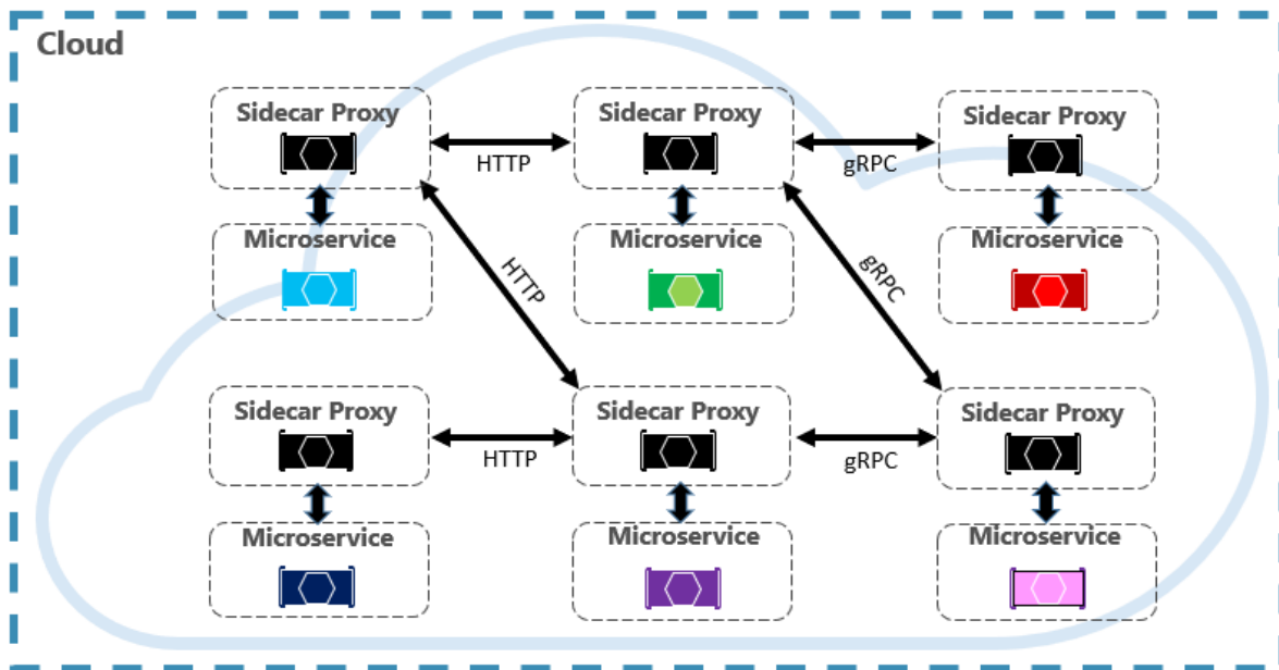
Figure 4-24. Service mesh with a side car
