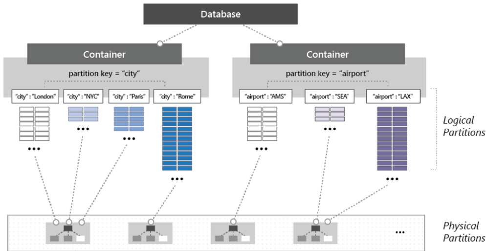
Figure 5-14: Cosmos DB partitioning mechanics
