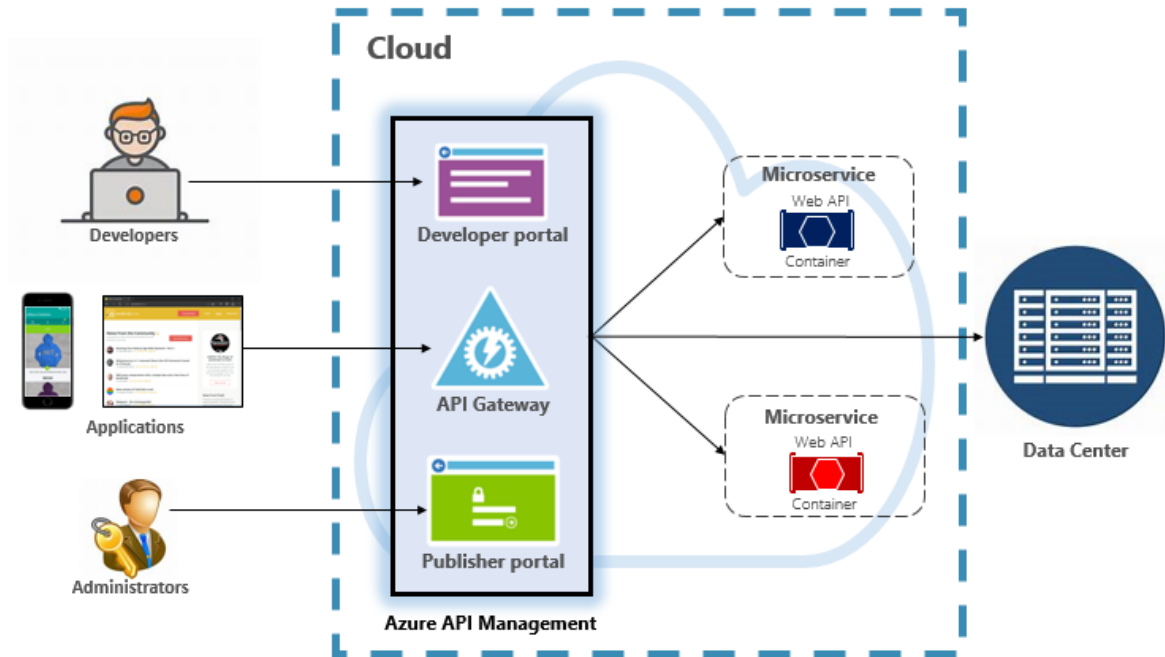
Figure 4-6. Azure API Management
