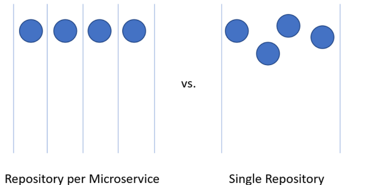
Figure 10-3 - One vs. many repositories.
