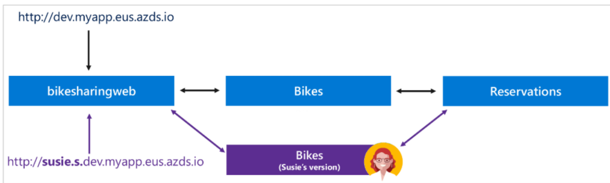
Figure 2-7. Developer Susie deploys her own version of the Bikes microservice and tests it.
