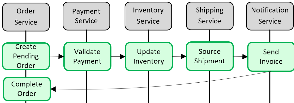
Figure 5-5. Implementing a transaction across microservices
