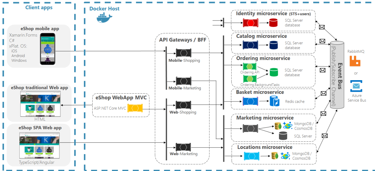
Figure 2-5. The eShopOnContainers Architecture.
