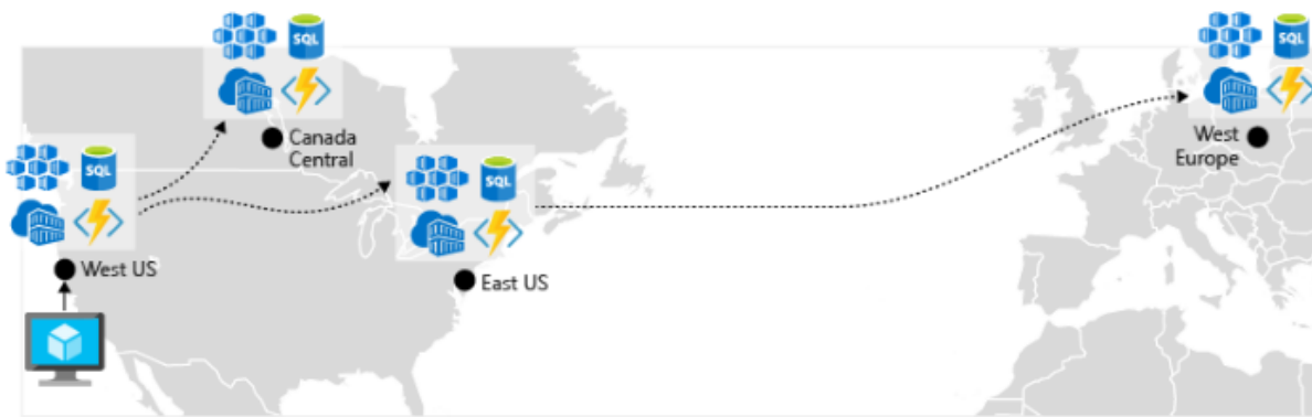
Figure 6-4. Replicated resources across regions
