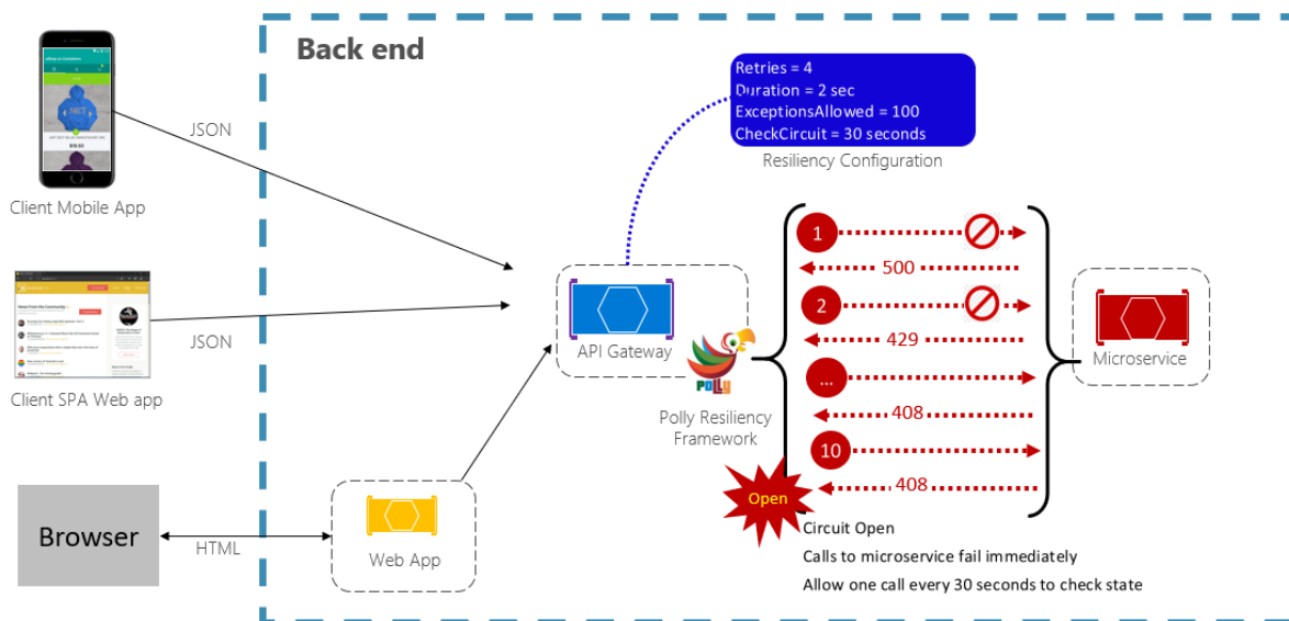
Figure 6-3. Circuit breaker pattern in action
