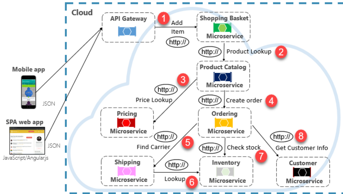
Figure 4-9. Chaining HTTP queries
